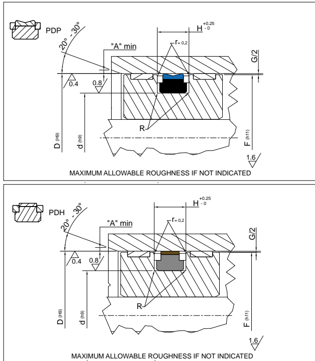
Piston Seal design guidelines
